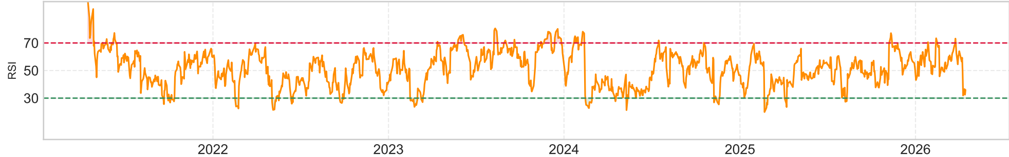
RSI (14-day) — Current: 36.0
