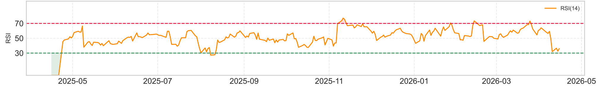
RSI (14-day Wilder) — Current: 36.0 [NEUTRAL]
